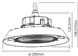
150W HiBLADE150/CT
