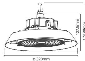
200W HiBLADE200/CT
