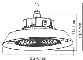
100W HiBLADE100
